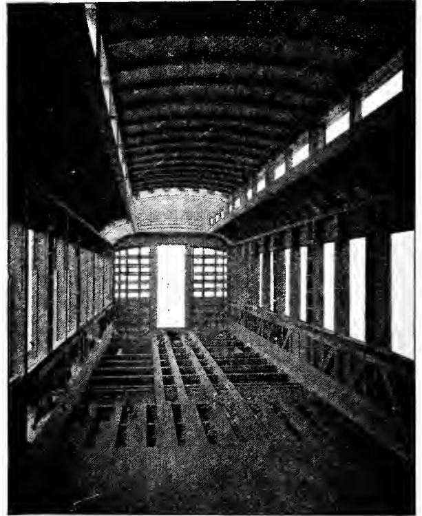
Fig. 533. Interior View, showing Sills, Bridging, Truss-plank, Trussing and Superstructure.
